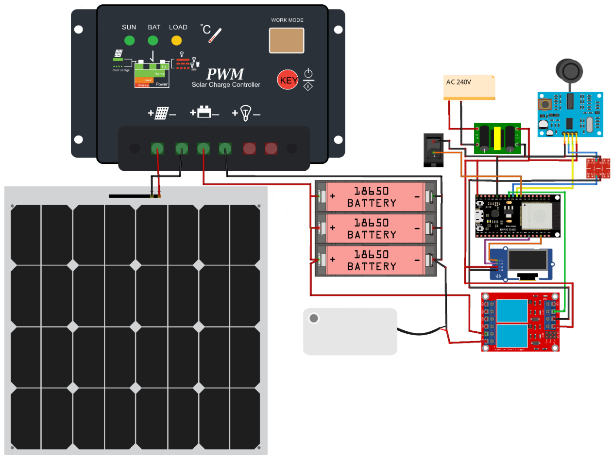
Figure 9: Circuit Diagram
