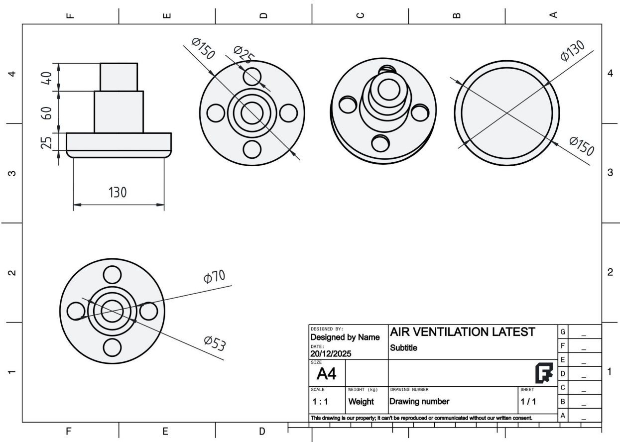
Figure 10: Air Ventilation part design
